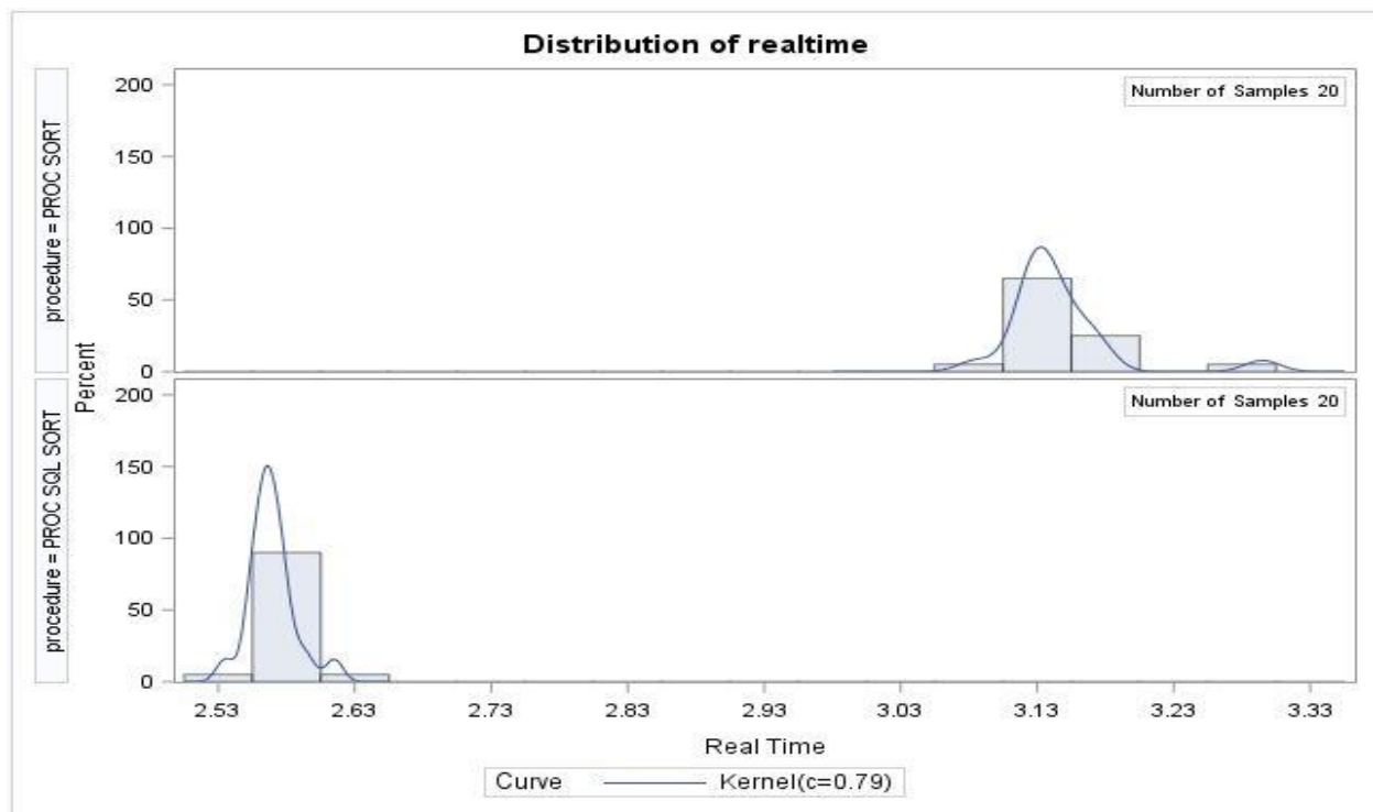
Figure 2. Relative Performance (Realtime) of SORT Procedure to SQL Procedure
