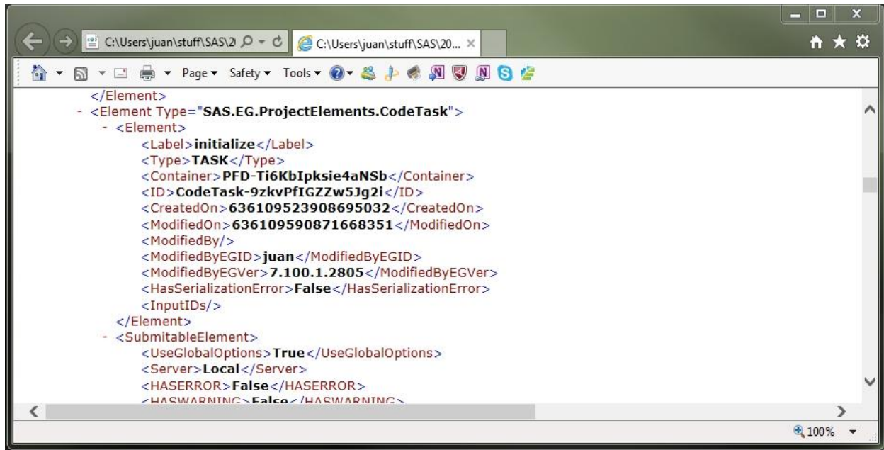
Figure 3. View of a SAS Enterprise Guide Project.xml File (Imbedded SAS Program)
