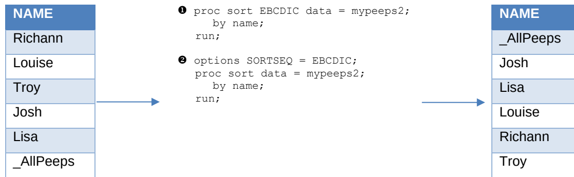
Sample Data 9: Sample Data Sorted Using Specified Collating Sequence, EBCDIC
